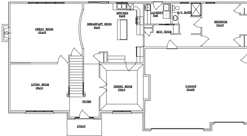
FIRST FLOOR LAYOUT
