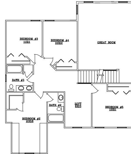
SECOND FLOOR
