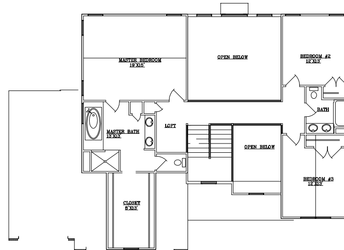
SECOND FLOOR LAYOUT
